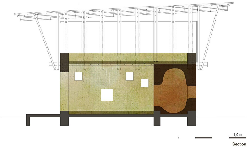
Section
