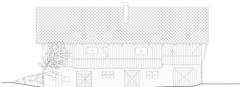
SOUTH ELEVATION
