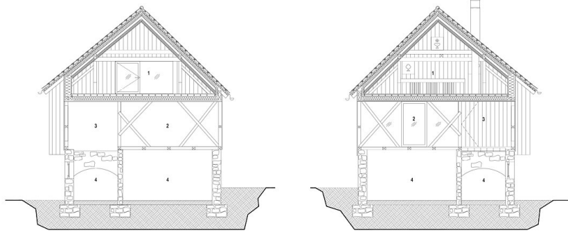
SECTION F-F
