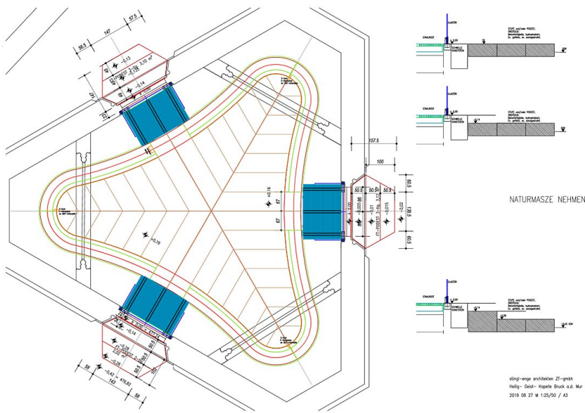
Detailplan Stufen
