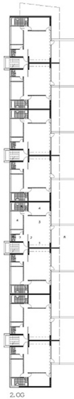
Grundriss OG1, OG2
