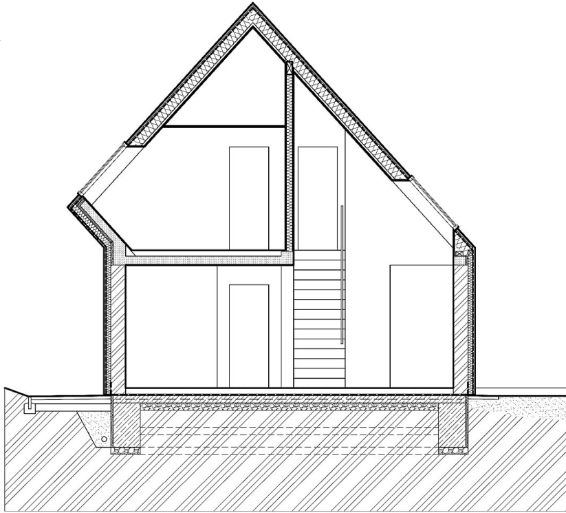
REZ 3-3
