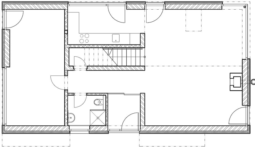
PŇDORYS PRIZEMIA
