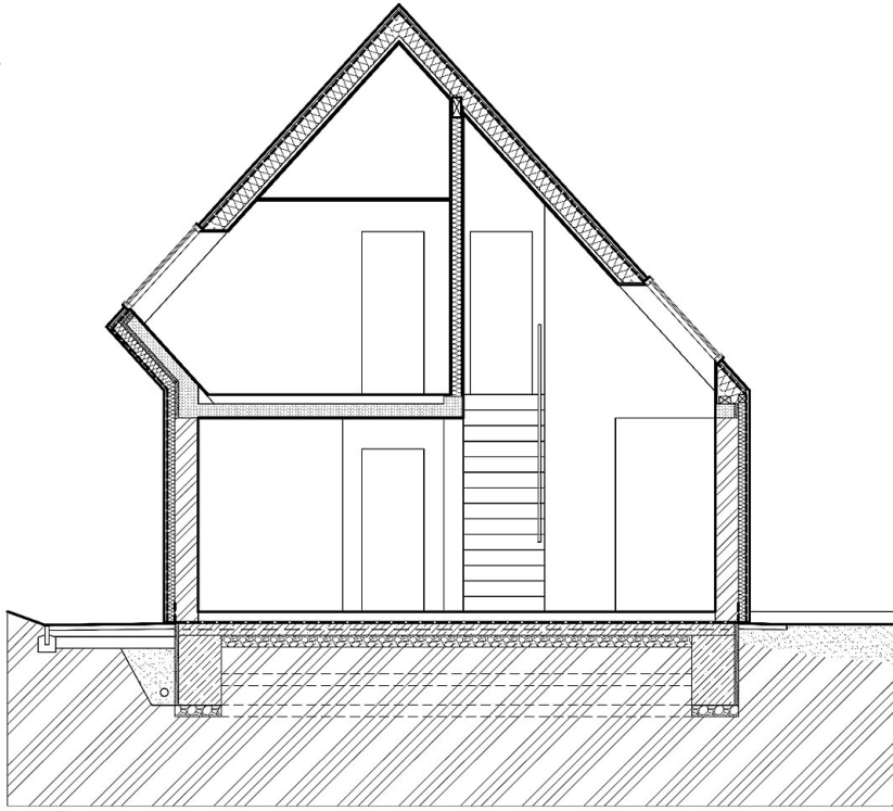
REZ 3-3
