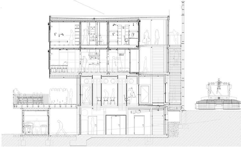
DETAILSCHNITT APARTMENT
