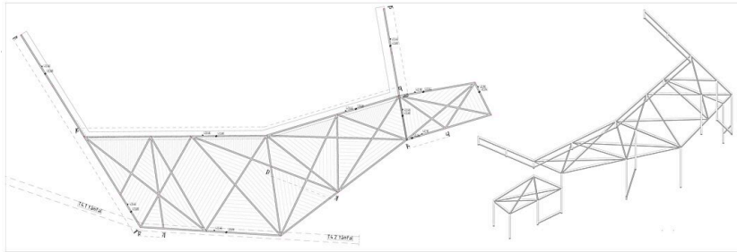
plan of the steel pergola
