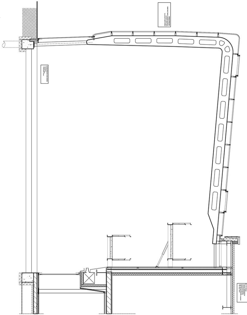
detail hortus
