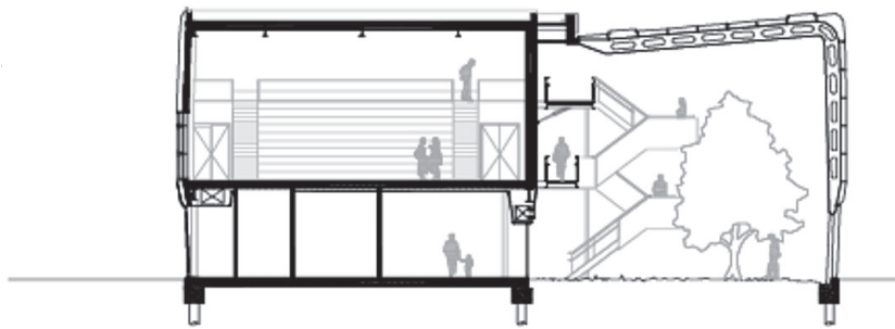
section 1
