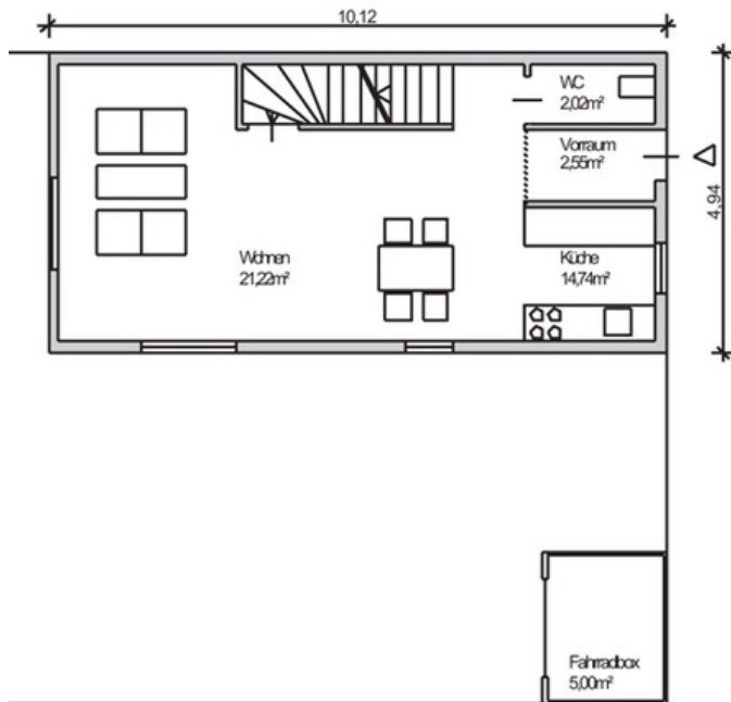
ERDGESCHOSS 40,53m 2
