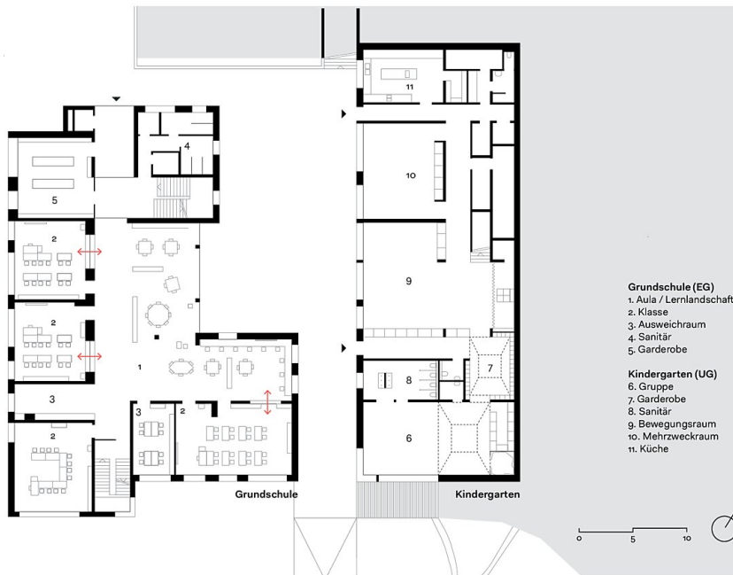
Grundriss EG-UG
