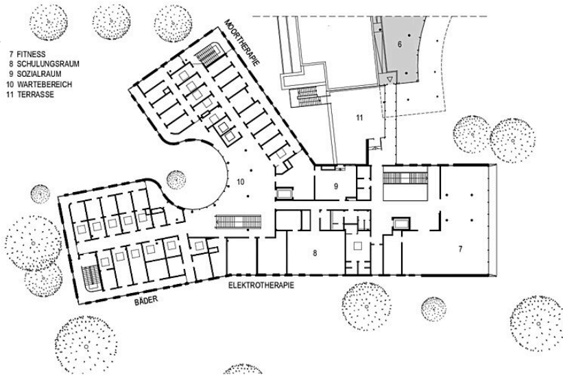
GRUNDRISS 1.0G
