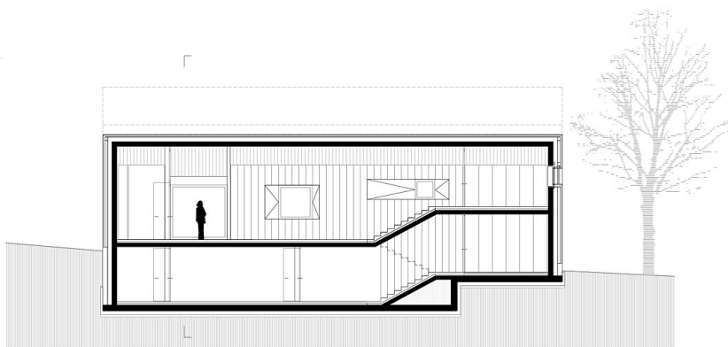
cross section 1-1
