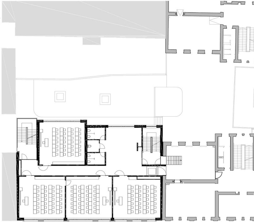
Grundriss OG2/3
