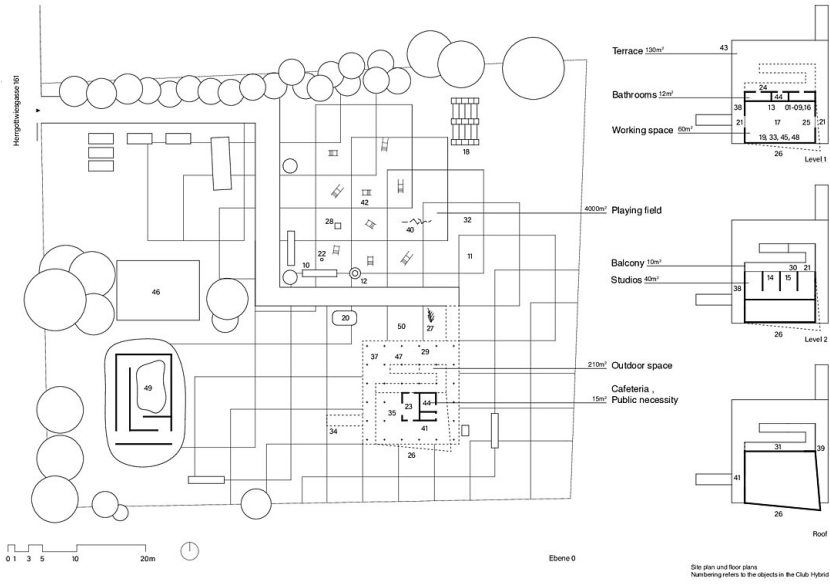
Club Hybrid 2021 ©Pretterhofer Rieper Siteplan And Floorplans
