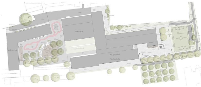
Freiraumplan
