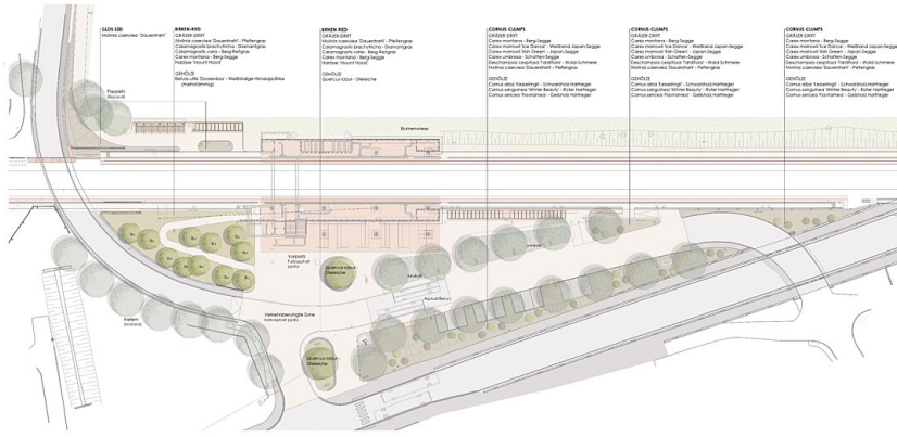
Freiraumplan
