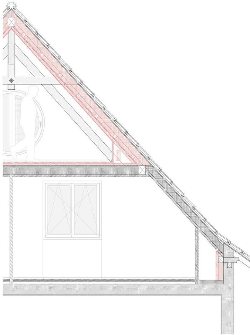
Detail 1b
