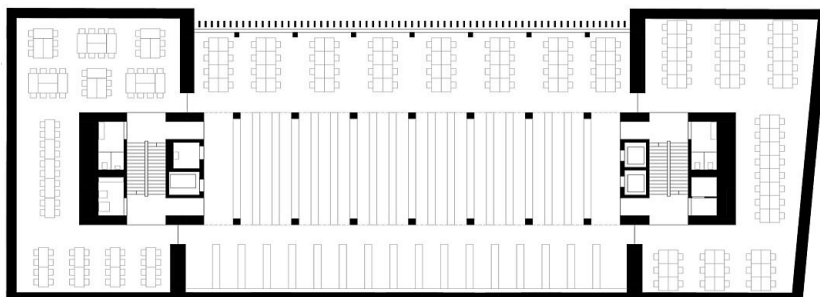
Grundriss OG2 &amp; OG4
