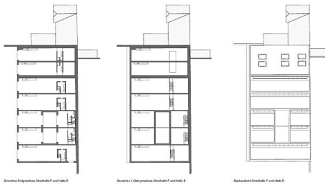
Grundriss Edgeschoss Shed F, Halle E
